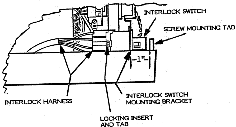
FIG. 3-27 INTERLOCK SWITCH
