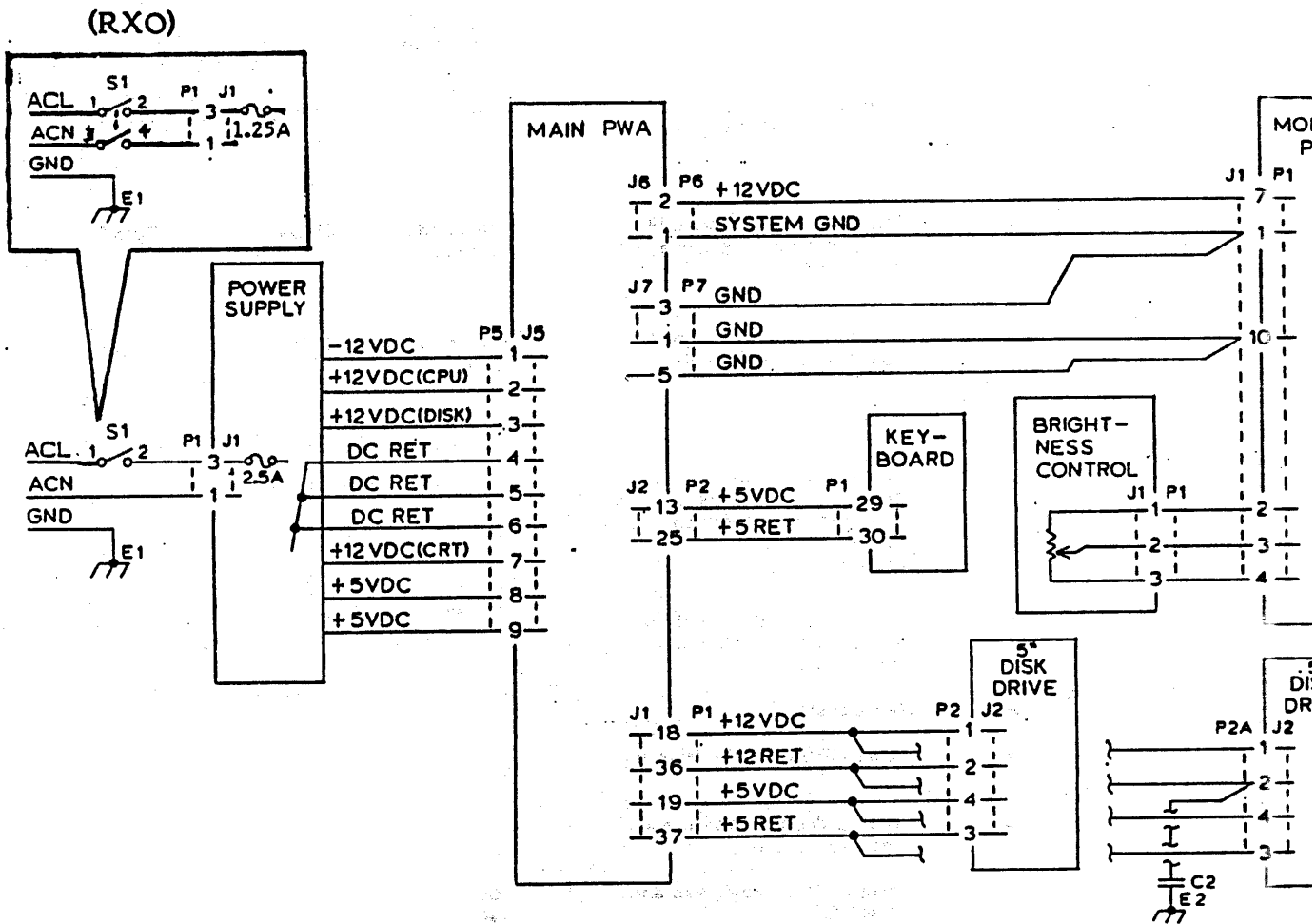
- AC/DC DISTRIBUTION
