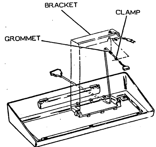
Figure 3-12 REMOVE HARNESS
